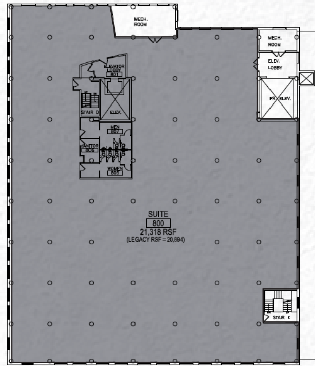
KEY PLAN
